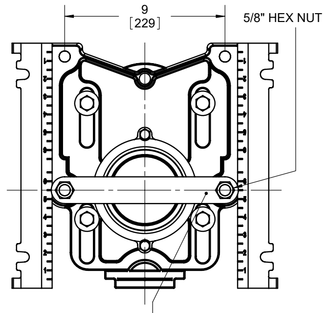
TEST BRACKET (P/N 070965 BRACKET ONLY)
