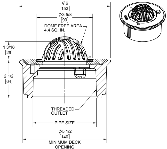
4" THREADED OUTLET
