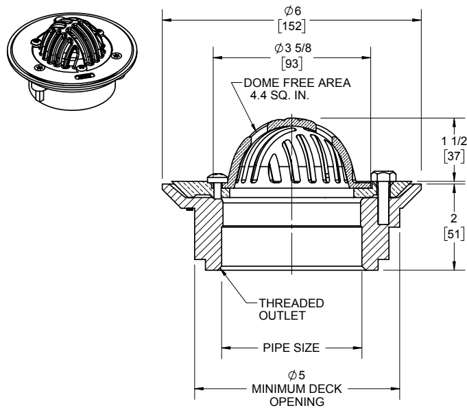
2" & 3" THREADED OUTLET
