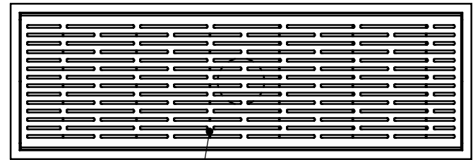
STANDARD GRATE 46610-LS GRATE LONGITUDINAL SLOT (FREE AREA = 38 in 2 /LF)
