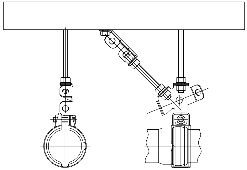
Example Installation
