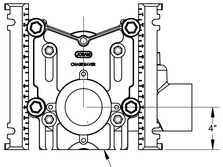
"TAS" OPTION FACEPLATE (010935)
