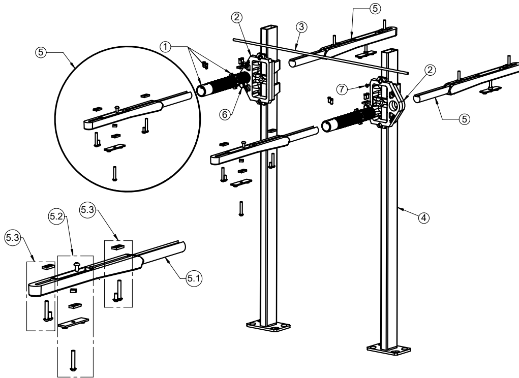
Pos. No. 5 - 17100-202 Arm Assembly
