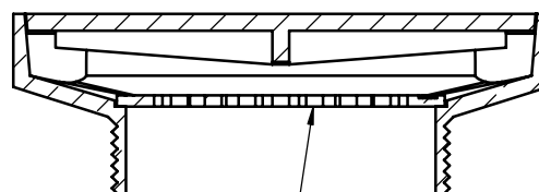
-88 SUPPLEMENTAL STRAINER (PN: 006815)
